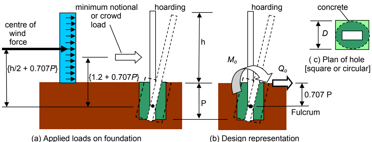
Figure D1 Post foundation
