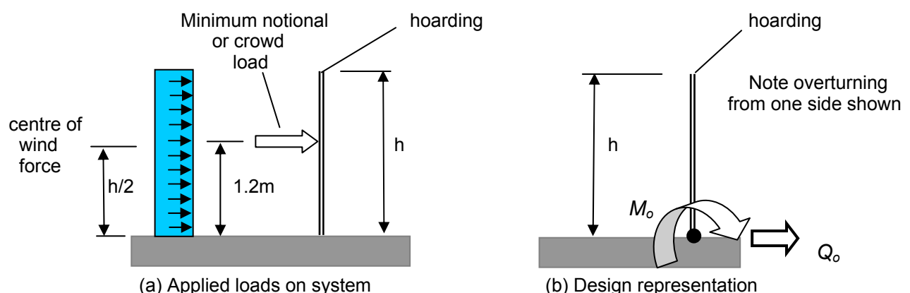
Figure 5 - Post design moment and shear
