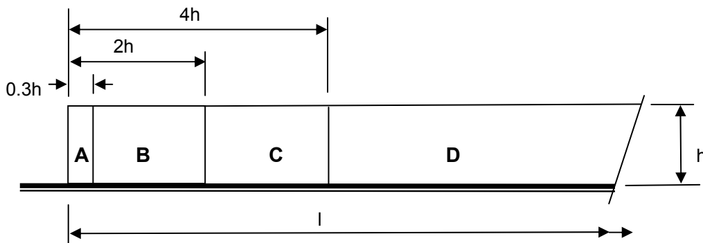
(a) Freestanding hoarding
