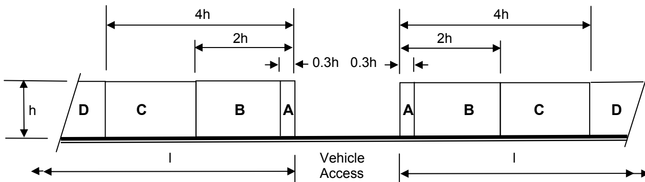
(b) Freestanding hoarding with vehicle access way
